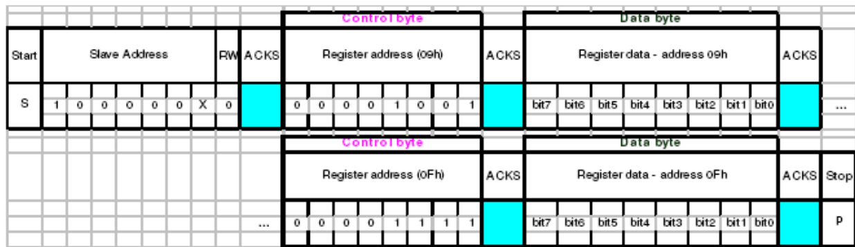
Figure 15: I²C multiple write
