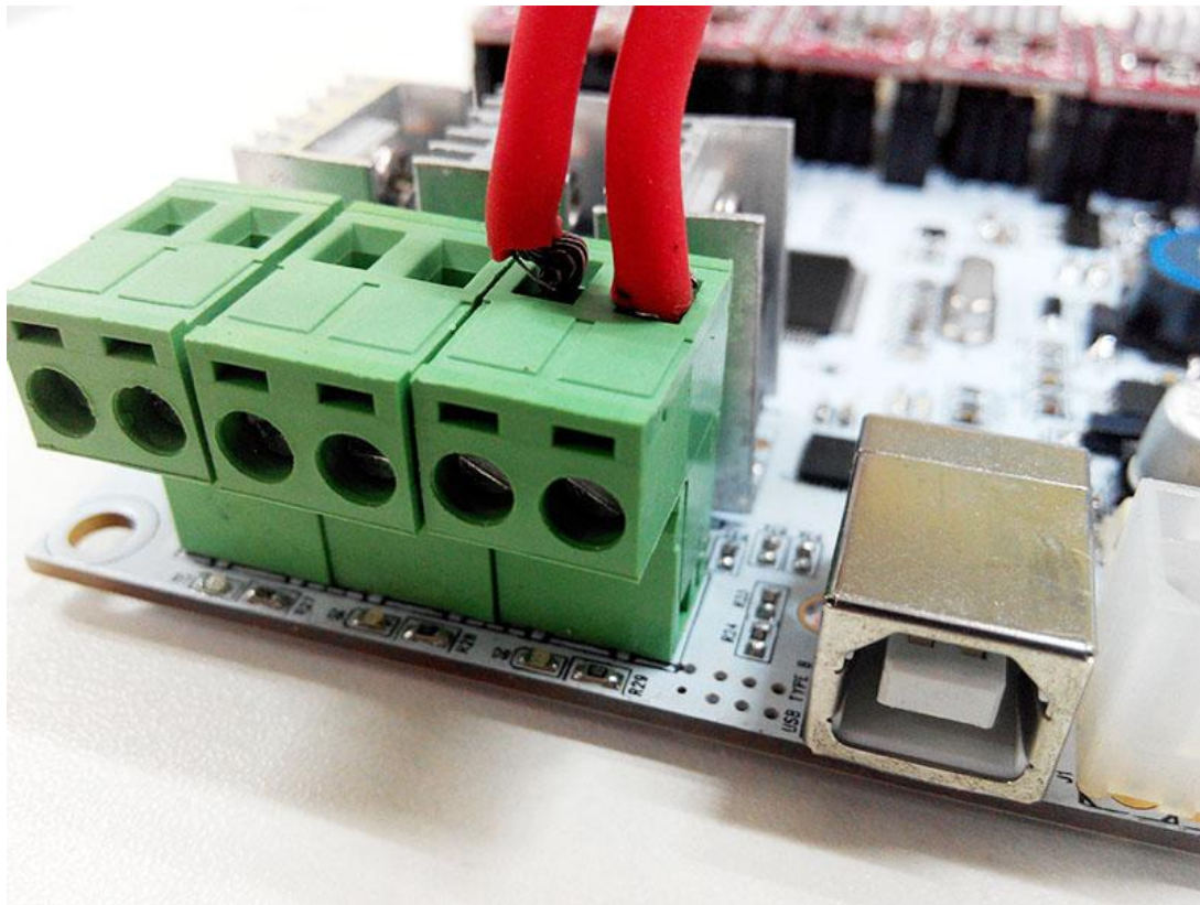
2) Connect heating wires for extruder 1.
