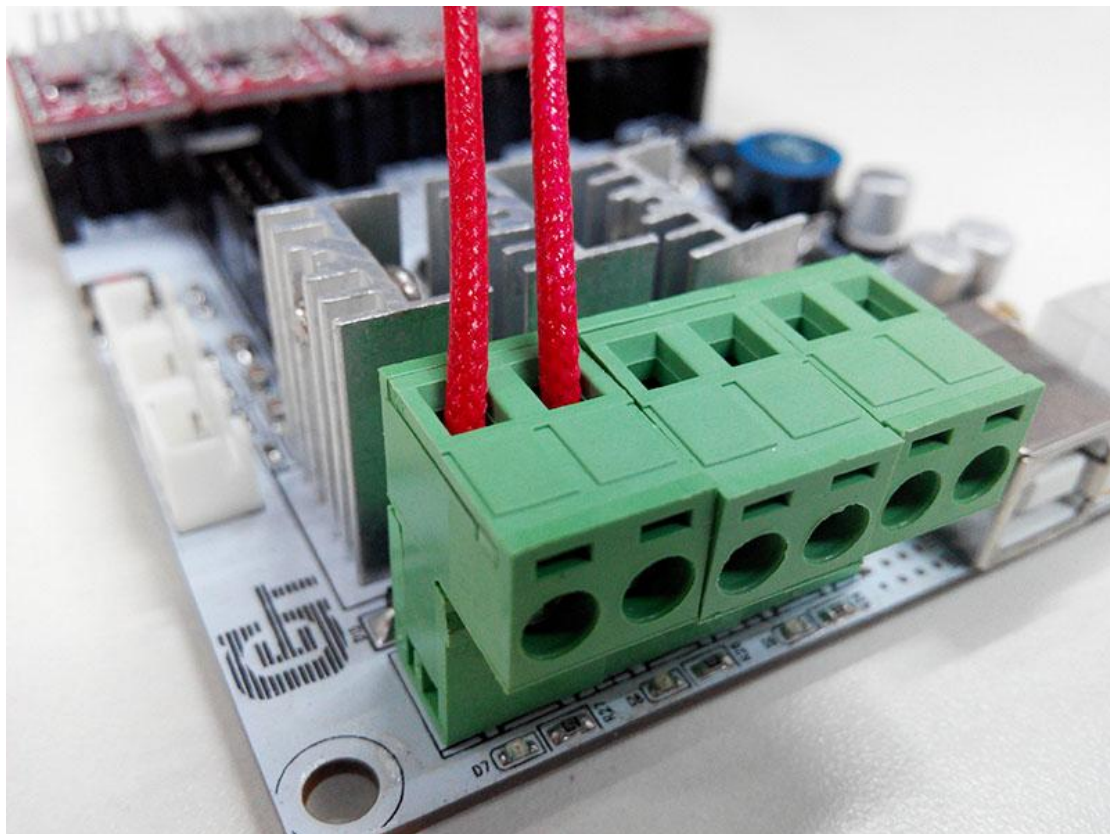
3) Connect heating wires for extruder 2.
